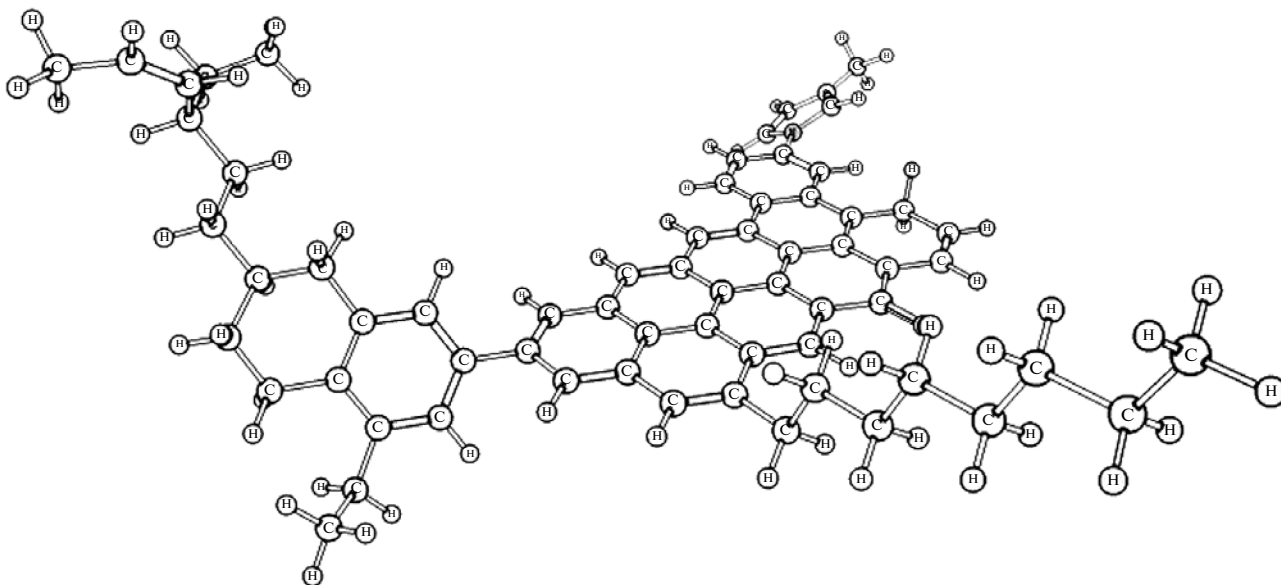
Fig. 1. Optimized structural model of bitumen from coal hydrogenation ( C_{65}H_{65}NO , with 12 aromatic and saturated rings).
