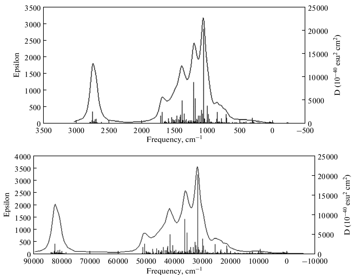
Fig. 2. IR spectrum of the structural model of bitumen.
